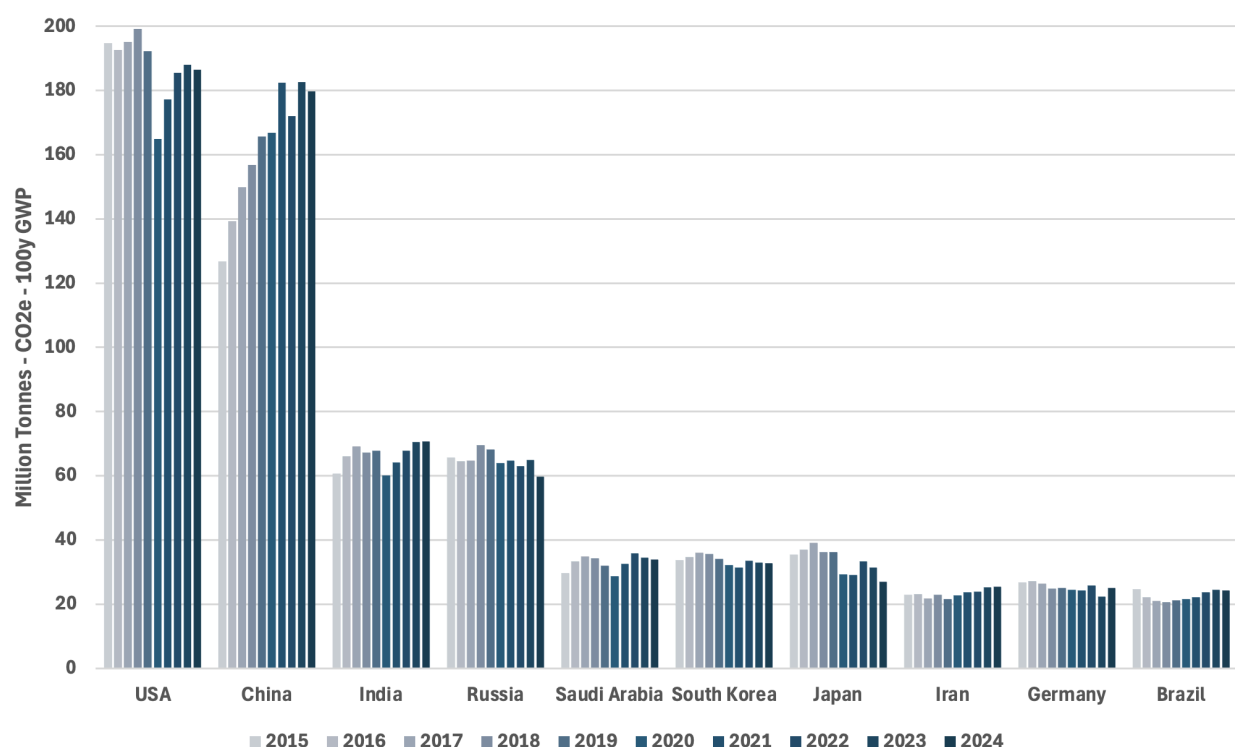
Figure 3 Top 10 global oil refining emitters, 2015-2024. Ordered by 2024 emissions.
