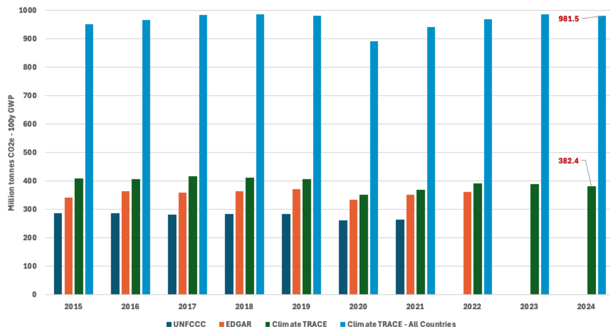
Figure 4 Comparison of global million tCO 2 e (100-year GWP) estimates in the refining sector amongst most annex 1 countries. UNFCCC (dark blue bars), EDGAR (orange bars), and Climate TRACE – comparable annex 1 subset (green bars), and Climate TRACE – All Countries (light blue bars) inventories are shown for the years 2015 to 2024. Some annex 1 countries with highly uncertain or irregular data, such as Russia, were not included in the first three data aggregations for a more accurate comparison.
