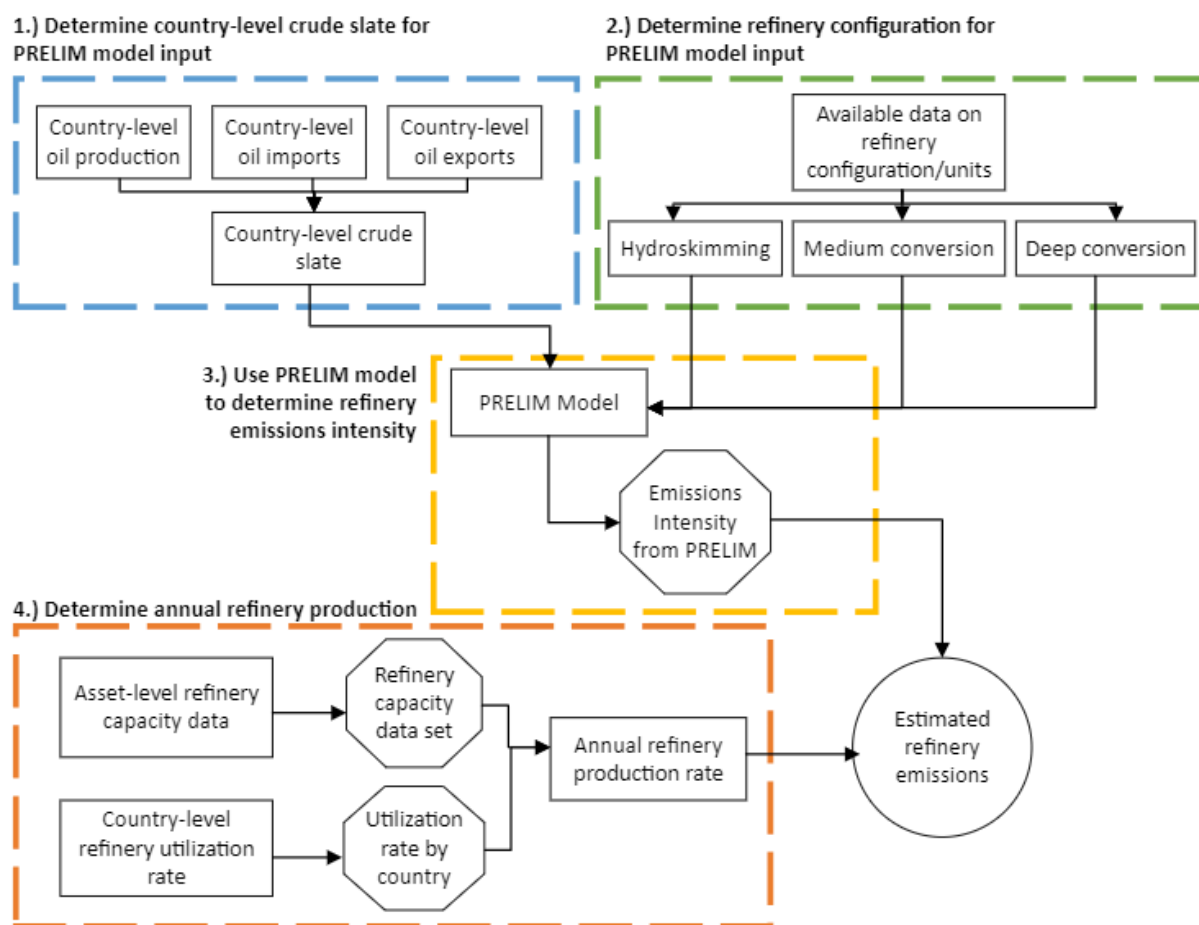
Figure 1 Refinery emission estimate methodology flowchart.
