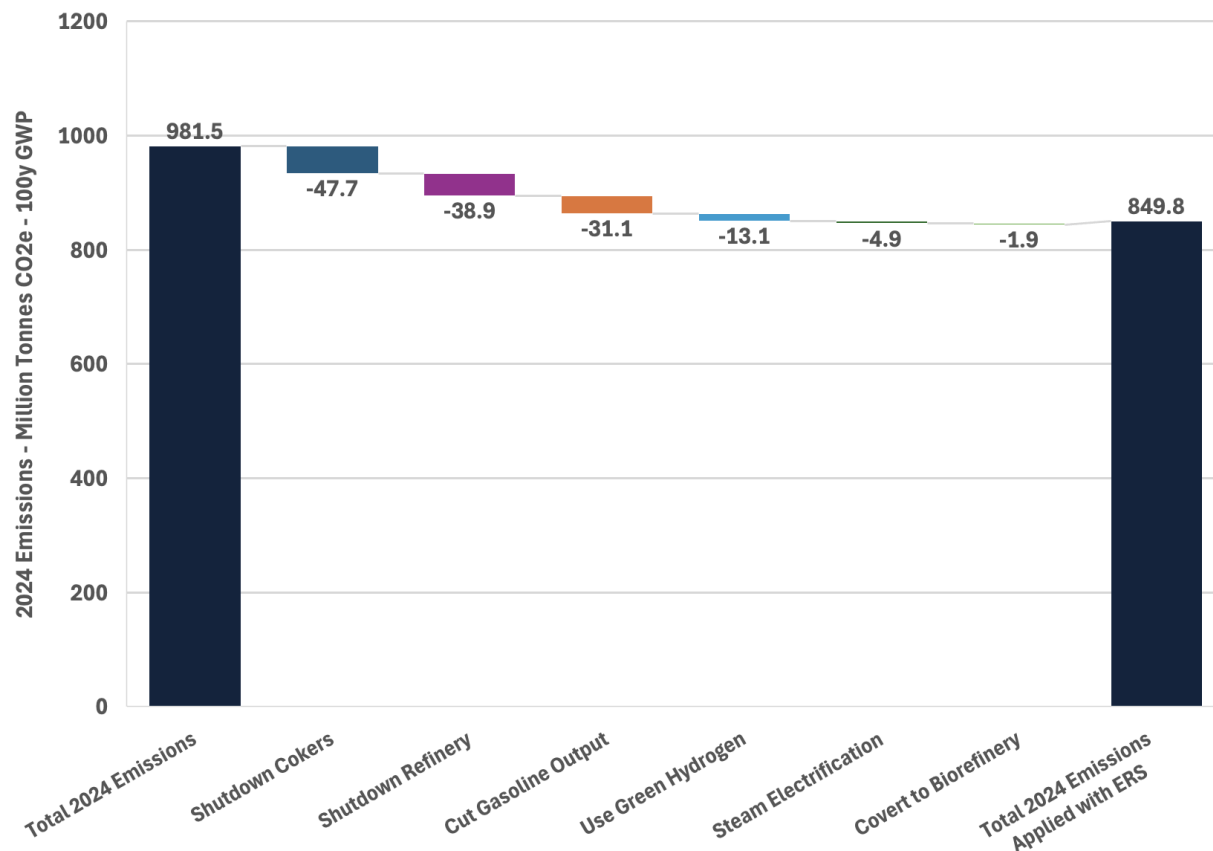
Figure 6 Waterfall chart demonstrating the emission reduction potential (million tCO 2 e 100-year GWP) contributed by each primary emission reduction strategy in 2024.
